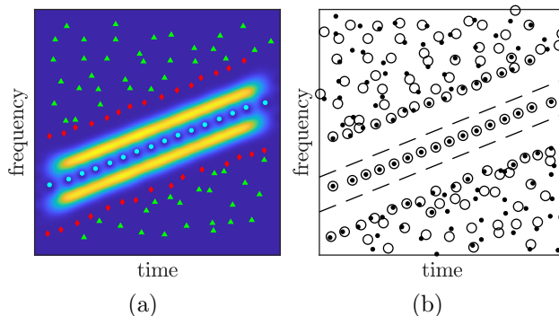
Figure 4: (a) Spectrogram of a signal with two parallel linear chirps contaminated by real WGN. Cyan dots correspond SZs of the SS kind, green triangles to those of the NN kind, while red diamonds represent SZs of the SN kind. (b) Position of SZs: Circles and dots indicate the position of the SZs corresponding to two different noise realizations. Dashed lines denote the instantaneous frequency associated with each chirp.
