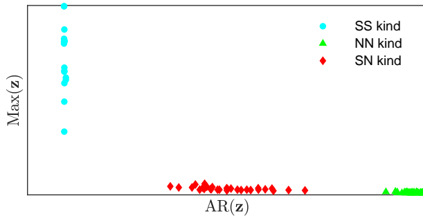
Figure 7: (a): Feature space of \text{AR}(\mathbf{z}) and \text{Max}(\mathbf{z}) . Each point represents one SZ of the spectrogram of the parallel chirps signal displayed in Fig. 4 (a). The markers and colors of the SZs correspond to SZ shown in Fig. 4 (a).
