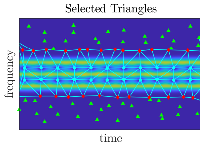
Figure 11: Delaunay triangles selected by applying the technique described in Sec. 7.2, based on the classification of spectrogram zeros. Blue dots denote SZs of SS kind, green triangles those of NN kind, and red diamonds those of SN kind.
