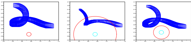
Fig. 1. Reachable sets of the original hundred dimensional system (left) and of its six dimensional and ten dimensional approximations (center and right). The circle on the left figure and the inner circle on the others represent the unsafe set \Pi_U . The outer circle on the center and right figure consists of the set of points whose distance to \Pi_U is smaller than the upper bound of the bisimulation metric.
